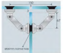
Glass to Glass Through Clamping Connector Dimension shown are for 60mm connecting rod length
