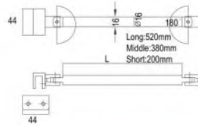
DM-73-5P | Material: SUS304/SUS316 Stainless Steel | Finish: Satin/Polish/PVD
