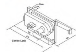
DM-411 Centre Lock (Single Action)
