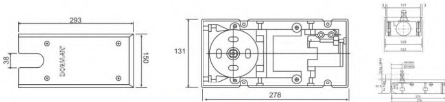
Technical drawing
