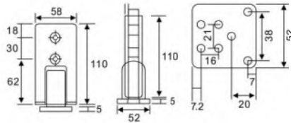
DM-SH720-1B 90° Wall Edge to Glass Fixing Microscler Bevel Corner for 8/10/12mm Glass SSS, PSS, Gold & Black SUS 304/316, Zinc, Brass
