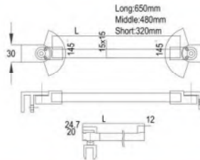
DM-73-6P | Material: SUS304/SUS316 Stainless Steel | Finish: Satin/Polish/PVD
