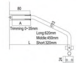
DM-73-4P | Material: SUS304/SUS316 Stainless Steel | Finish: Satin/Polish/PVD
