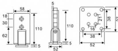
DM-SH720B 90° Wall to Glass Fixing Microscler Bevel Corner for 8/10/12mm Glass SSS, PSS, Gold & Black SUS 304/316, Zinc, Brass
